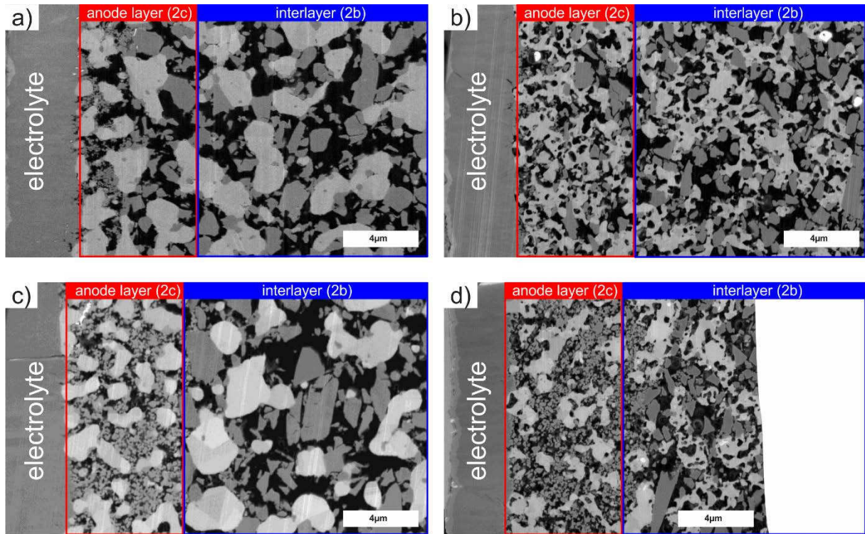
Figure 4: Comparison of the microstructures of cells with a (a, b) Ni/YSZ anode; (c, d) Ni/GDC anode; (a, c) before redox cycling; (b, d) after 35 short-term redox cycles in the temperature range of 300–700 °C (Ni = bright phase, YSZ or GDC = gray phase, pores = black). Cells were cooled down in the reduced state.
