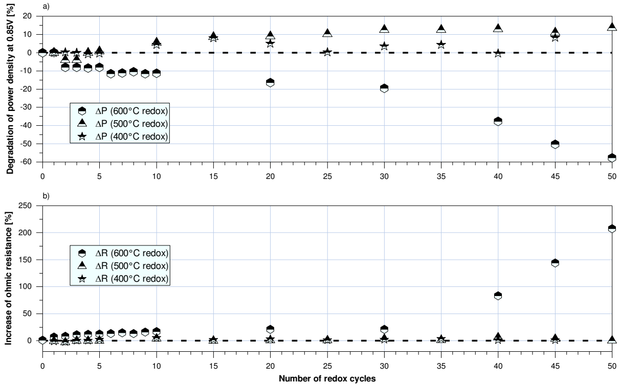
Figure 8: a) Degradation of the power density of an MSC test cell with a Ni/GDC anode as a result of b) ohmic resistance increasing with the number of redox cycles at 600 °C, 500 °C, and 400 °C; data recorded at 600 °C cell temperature each.
